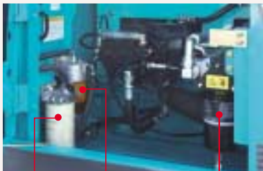
Main fuel filter Pre-fuel filter (with built-in water separator) *Optional for NZ Engine Oil Filter
