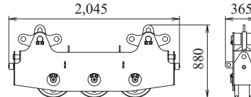
Upper Spreader (for Crane) Weight: 475 kg
