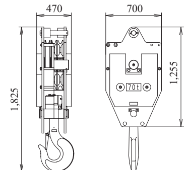
70 t Hook Weight: 1,200 kg
