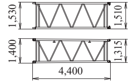
4.3 m Taper Jib Insert (Luffing Jib) Weight: 410 kg
