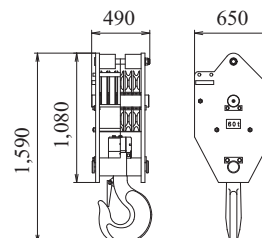
60 t Hook Weight: 700 kg
